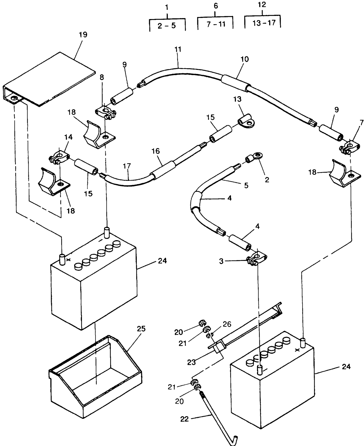
Figure 1. Batteries and Cables
