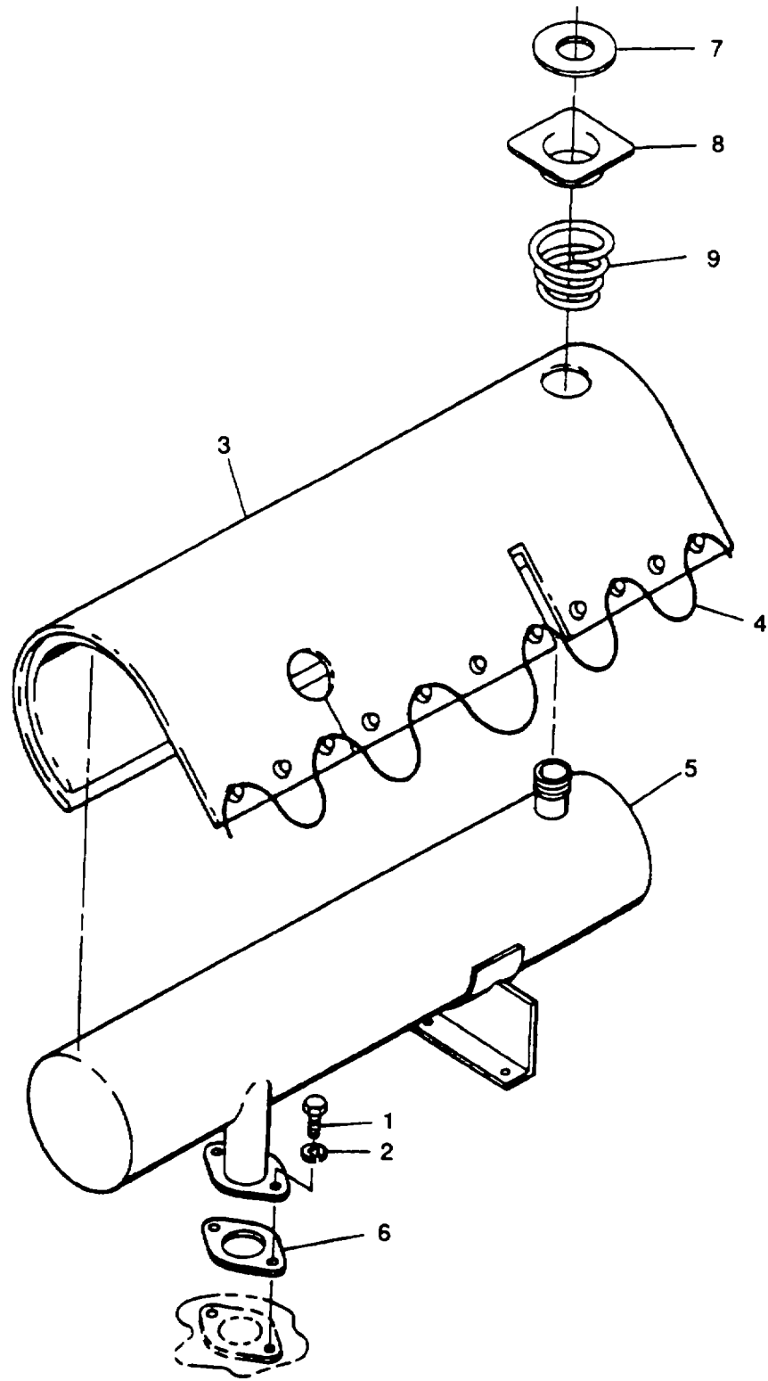
Figure 14. Muffler Assembly
