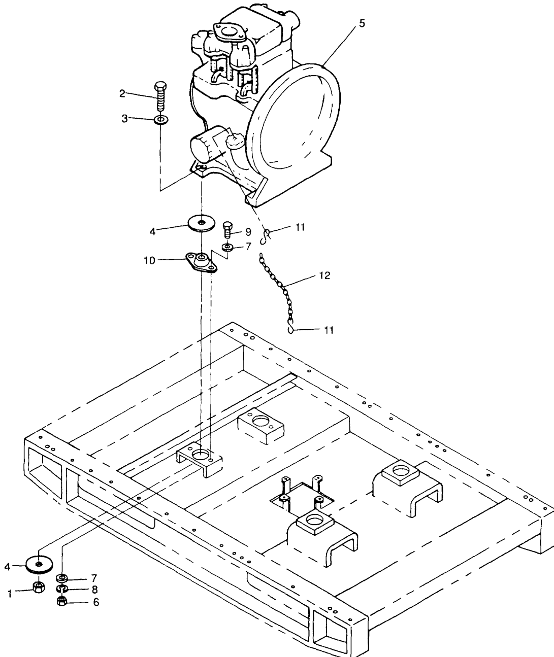
Figure 26. Engine Installation
