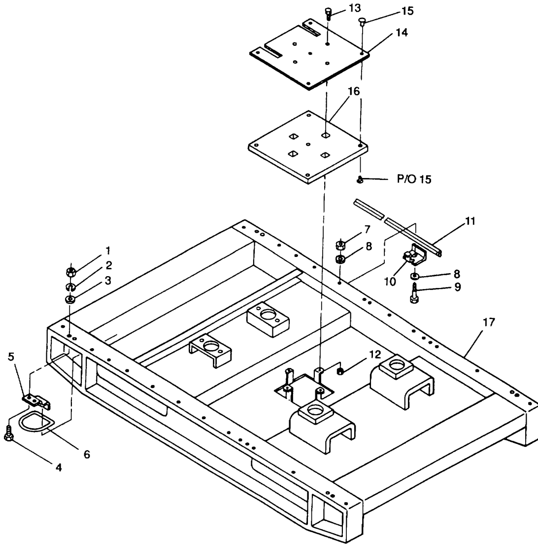
Figure 21. Skid Base Assembly
