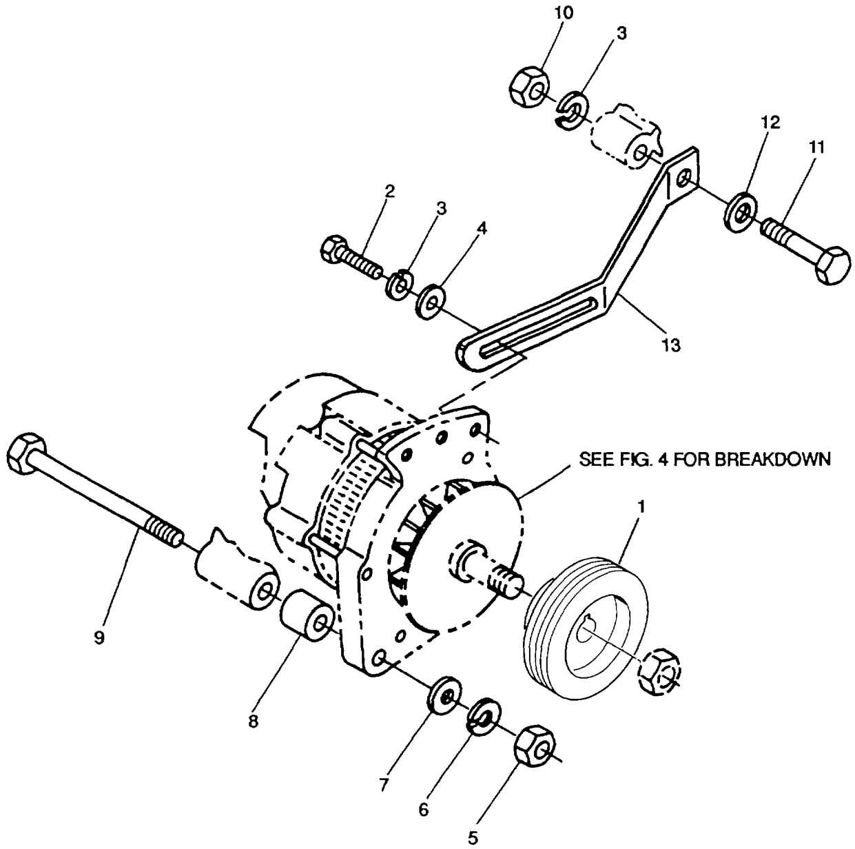
Figure 3. Alternator Installation
