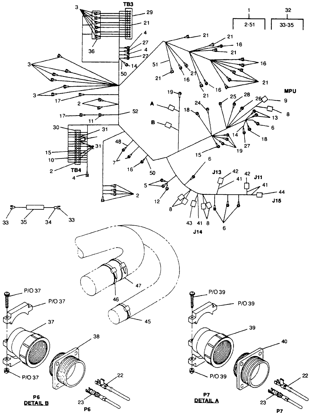
Figure 12. Output Box/Engine Harness Assembly
