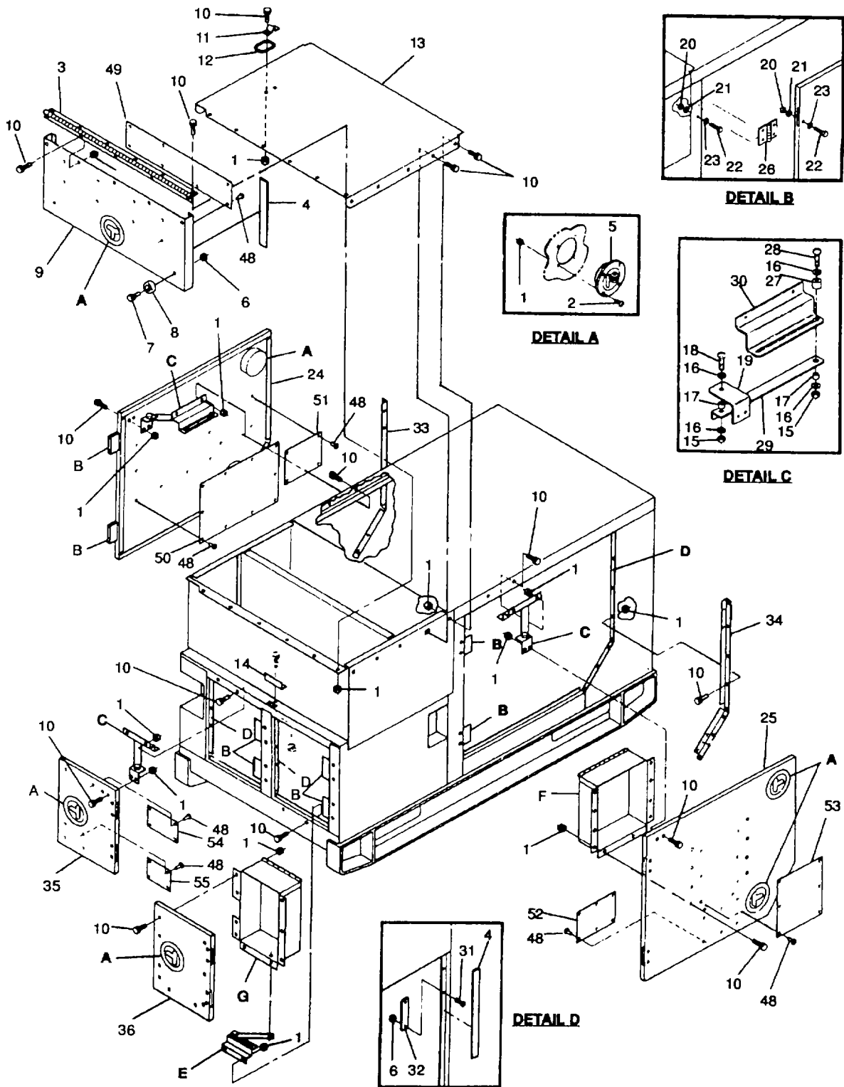
Figure 5. Access Doors and Covers (Sheet 1 of 2)
