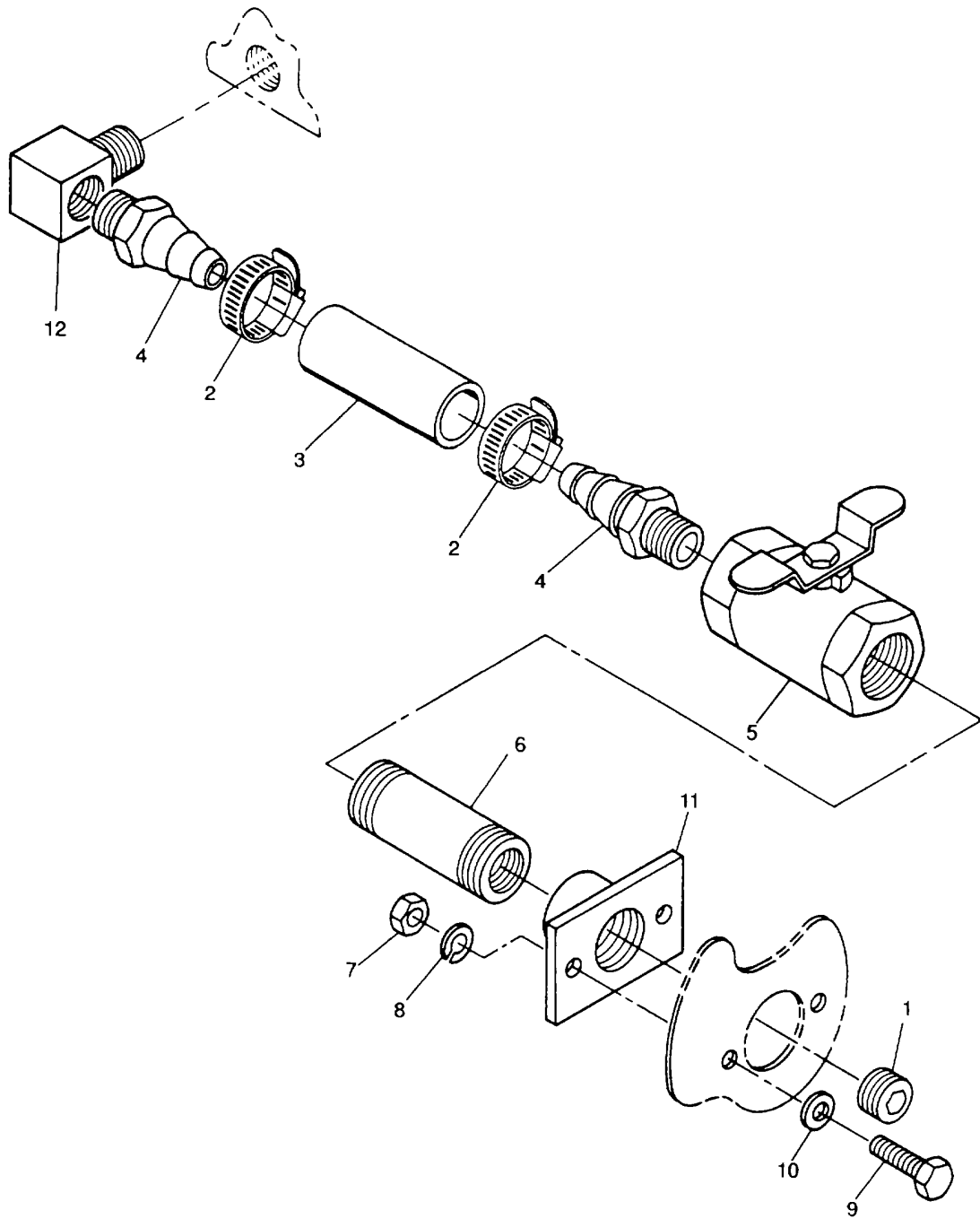
Figure 18. Oil Drain Line
