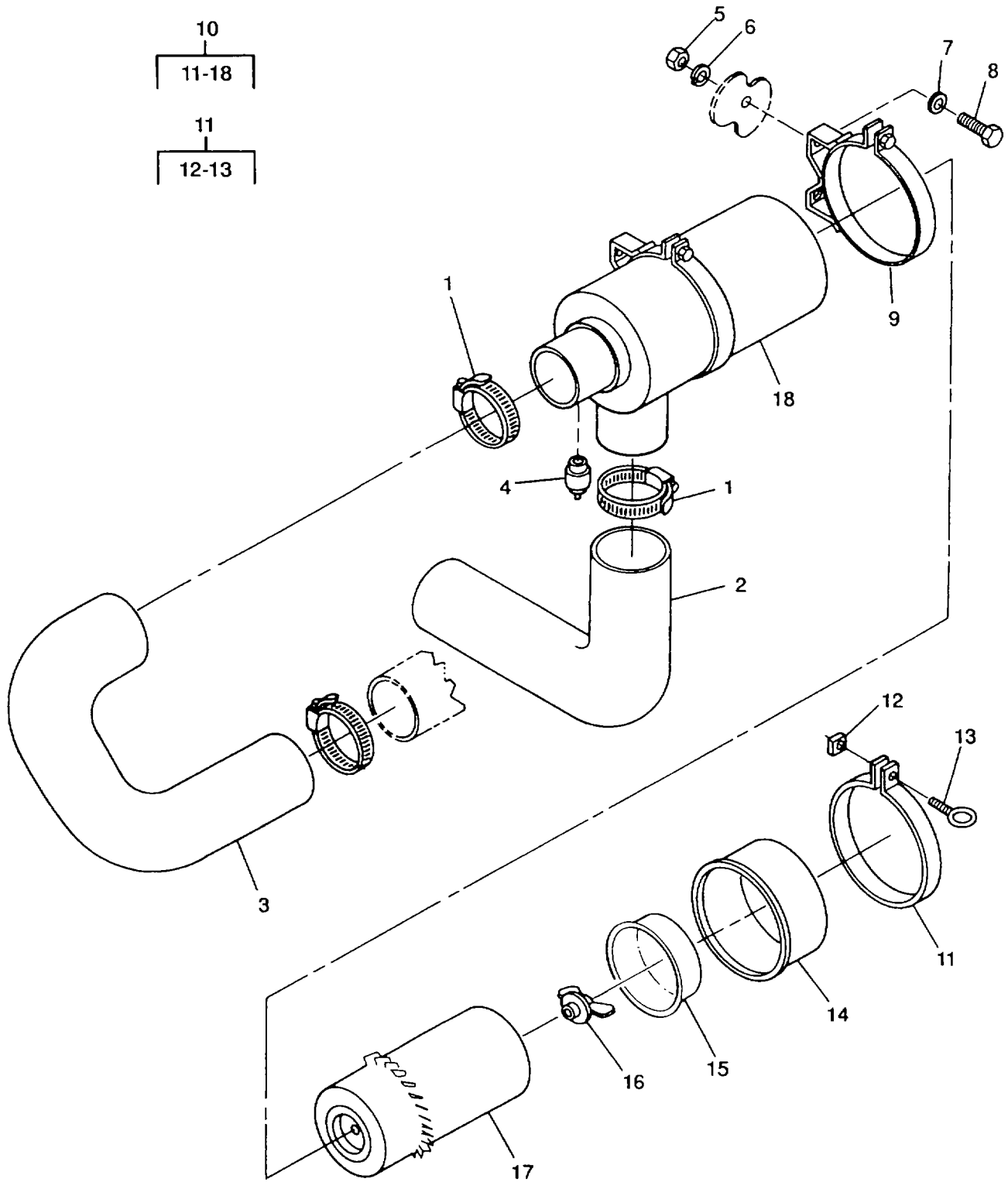
Figure 15. Air Cleaner Assembly
