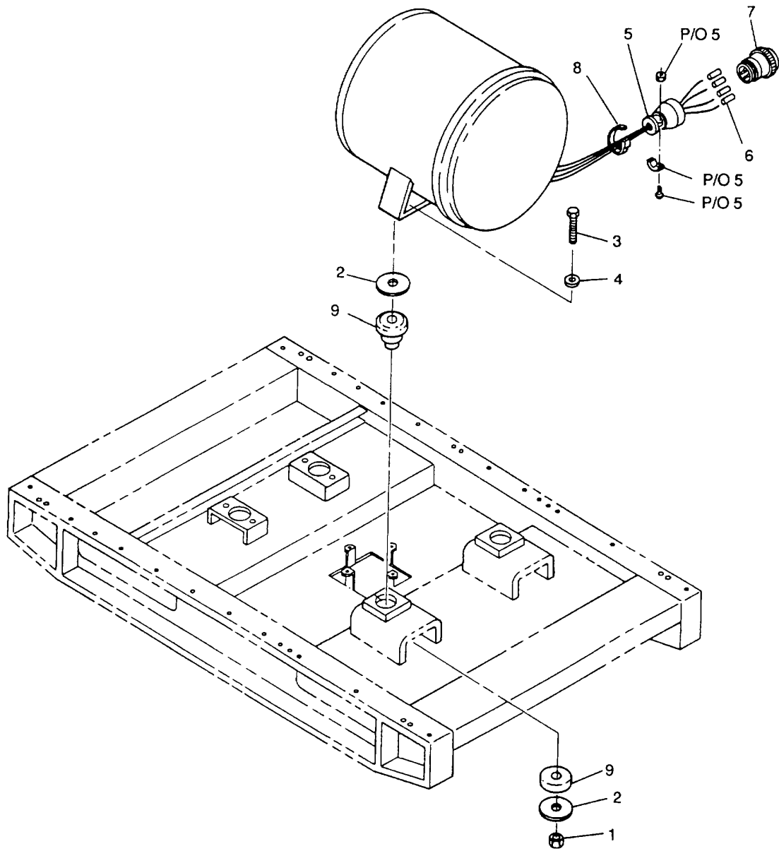
Figure 23. Generator Installation
