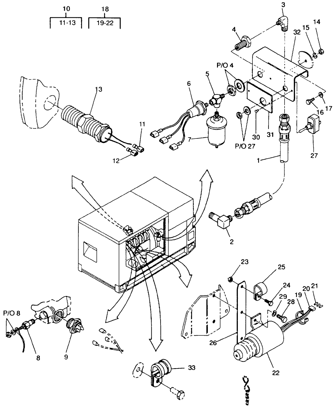
Figure 20. Engine Accessories
