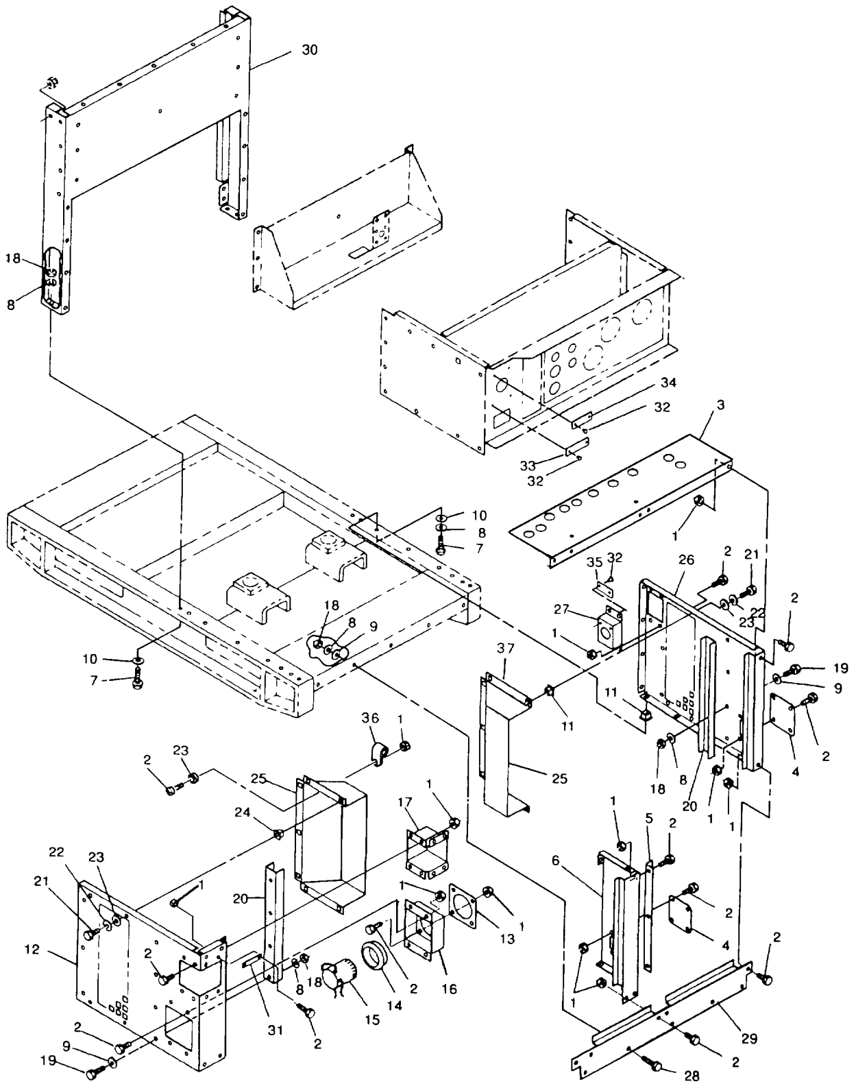
Figure 7. Rear Housing Panels
