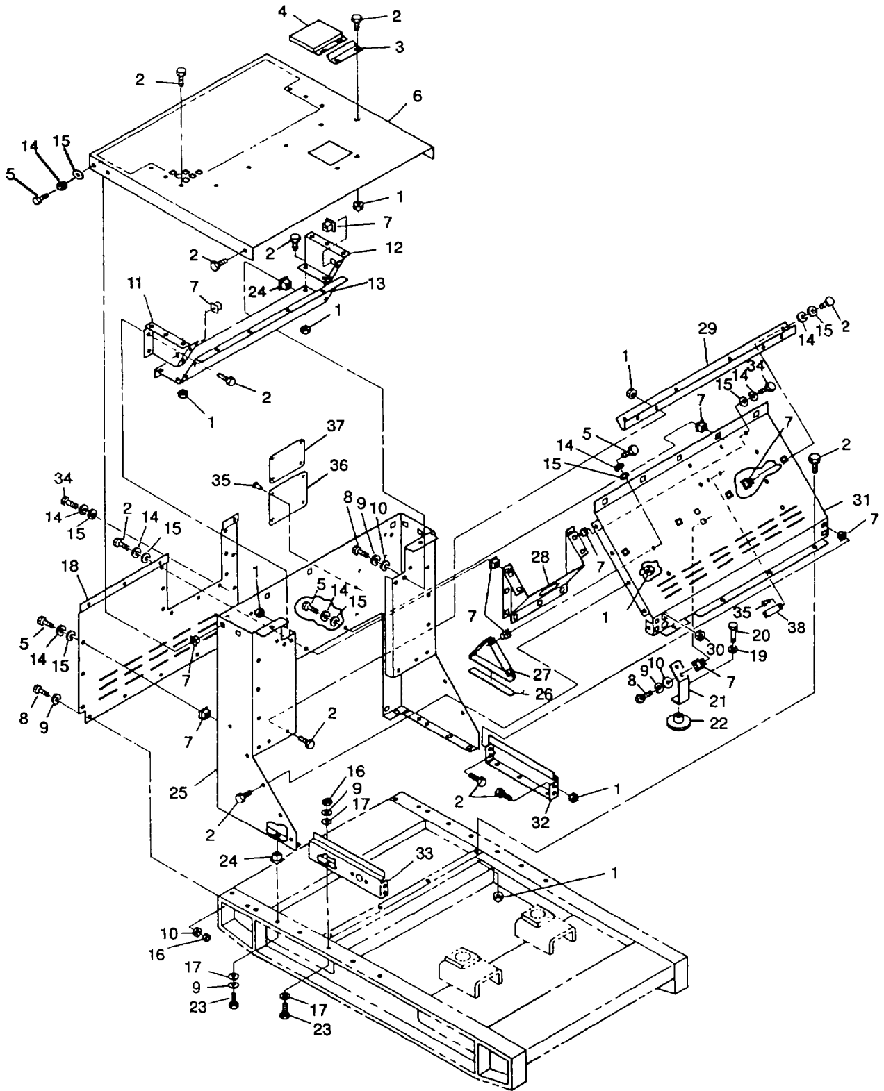
Figure 6. Front Housing Panels
