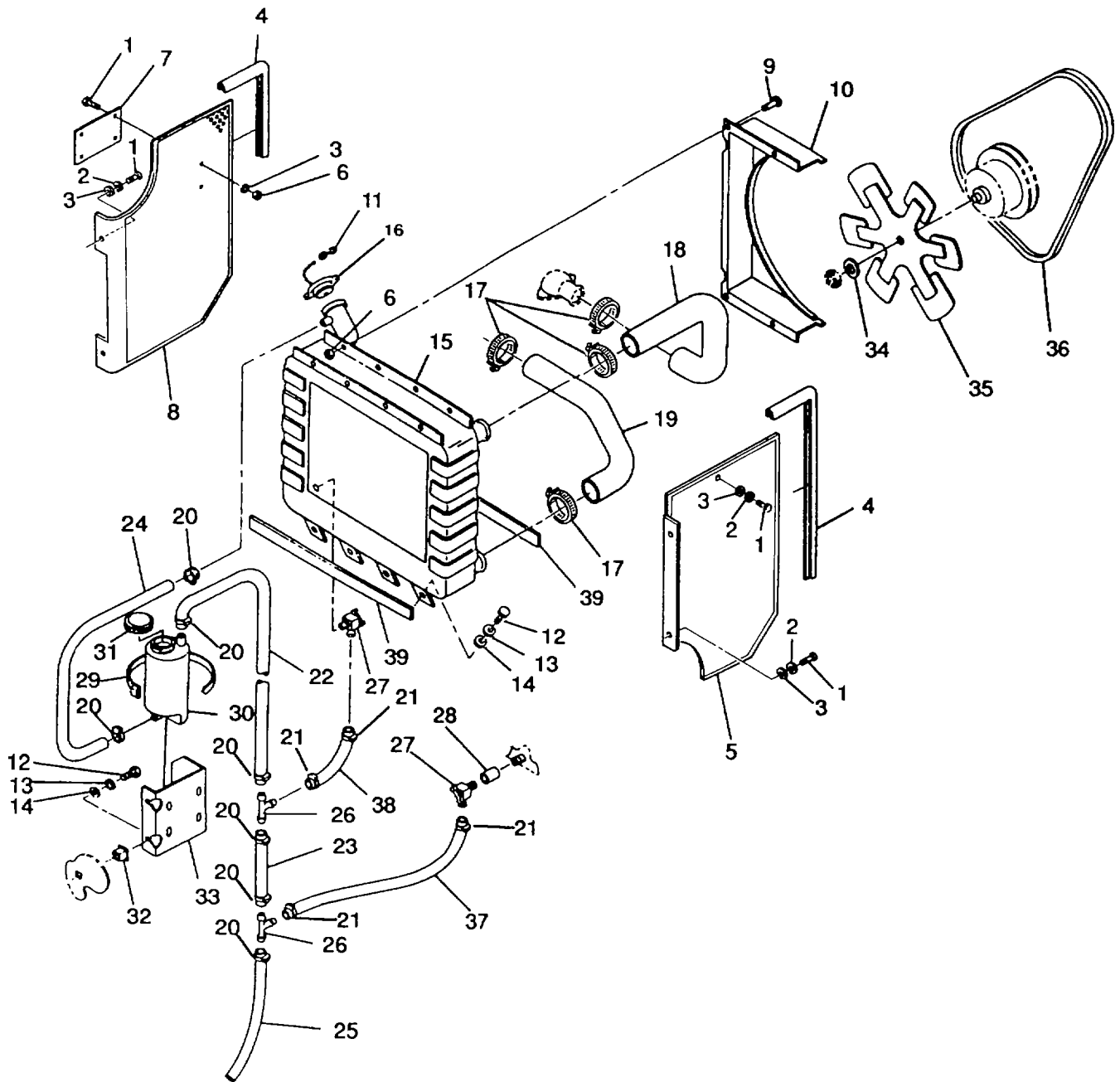
Figure 16. Radiator and Hoses
