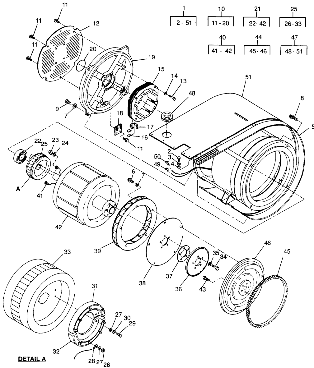
Figure 25. Generator Assembly, 400 Hz
