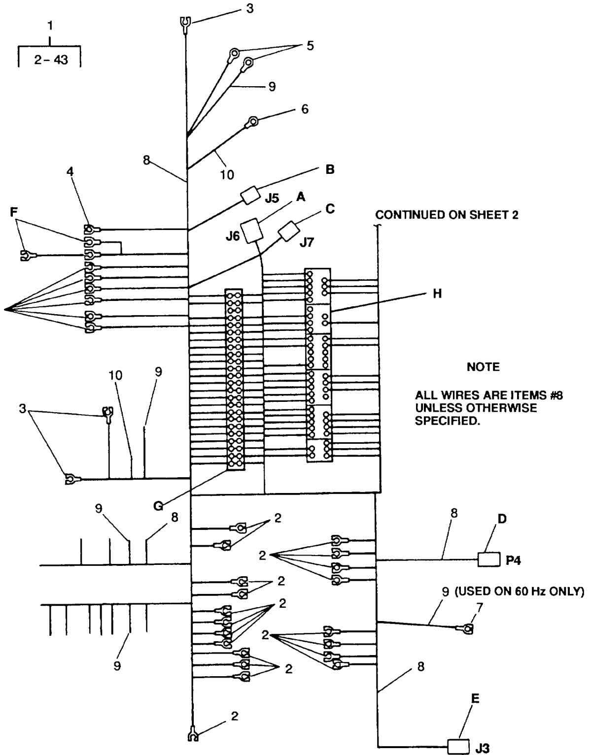
Figure 9. Control Box Harness (Sheet 1 of 4)
