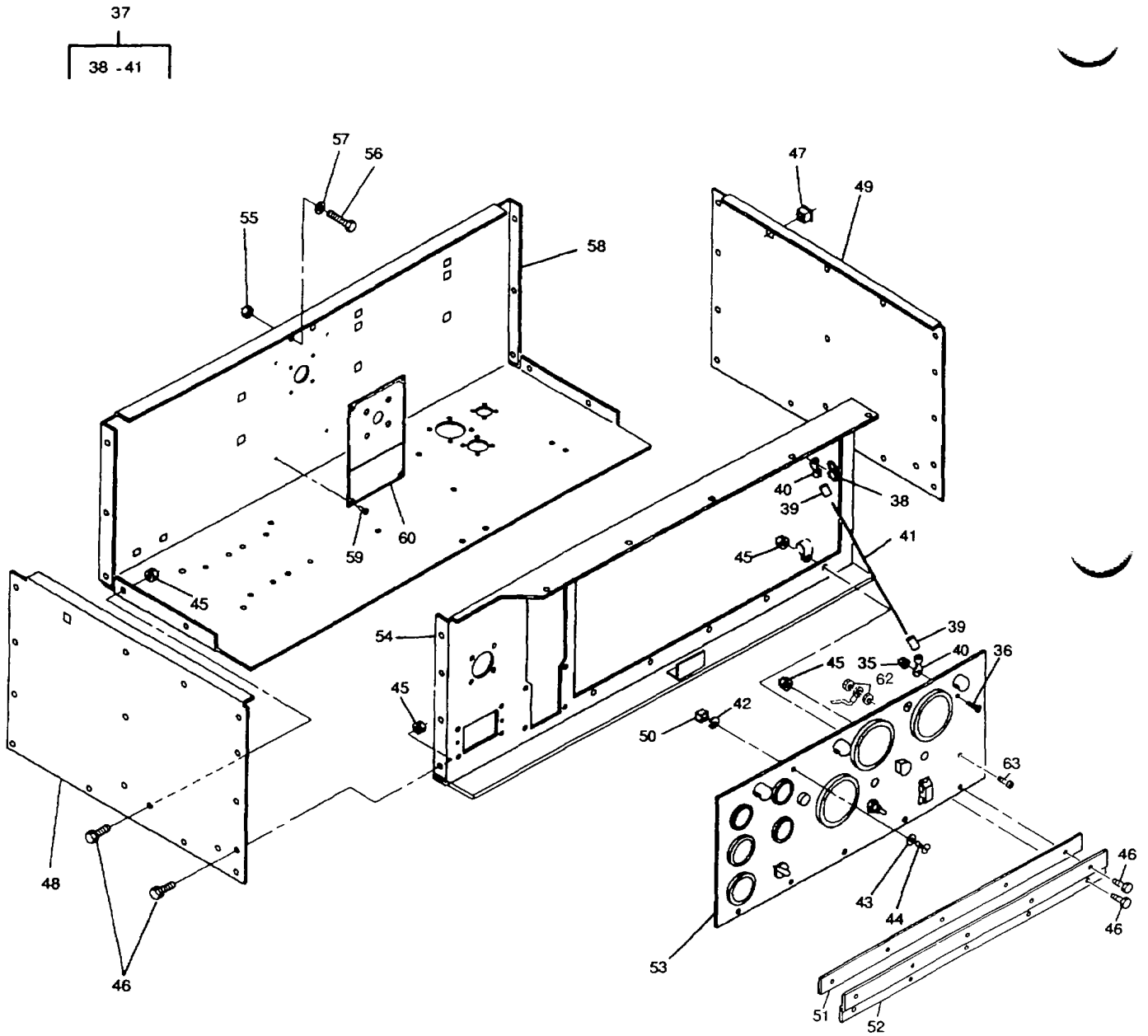
Figure 10. Control Panel and Box Assembly (Sheet 2 of 2)
