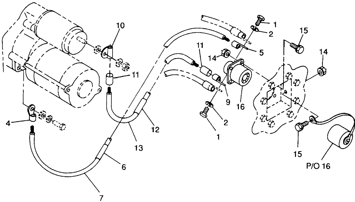
Figure 2. Slave Receptacle and Cables
