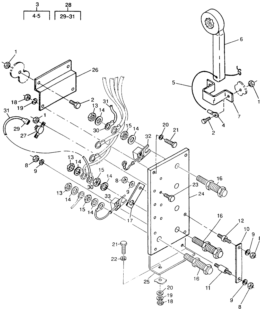
Figure 22. Load Terminal Board
