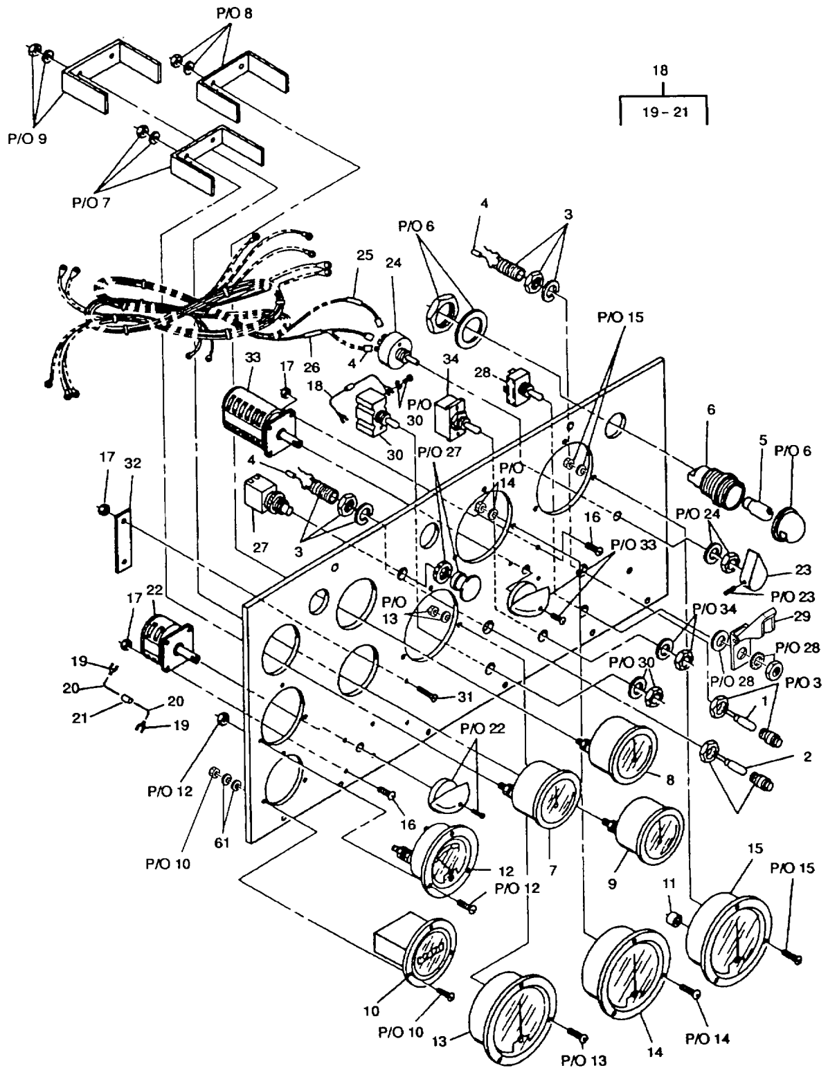
Figure 10. Control Panel and Box Assembly (Sheet 1 of 2)
