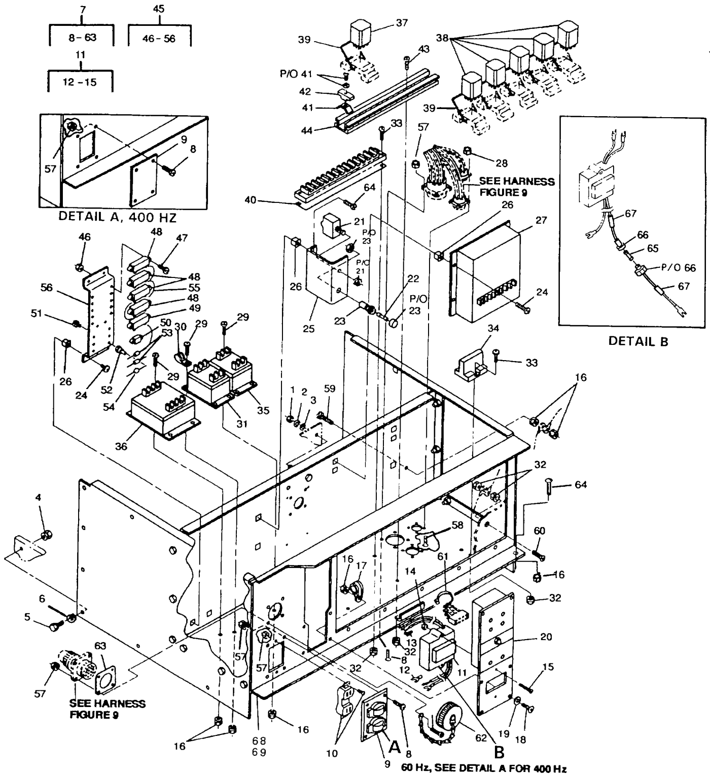
Figure 8. Control Box Assembly
